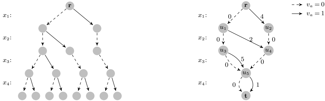
Figure 1 A decision tree and a DD for \mathcal{X} = \{\mathbf{x} \in \{0,1\}^4 : 7x_1 + 5x_2 + 4x_3 + x_4 \leq 8\} .
