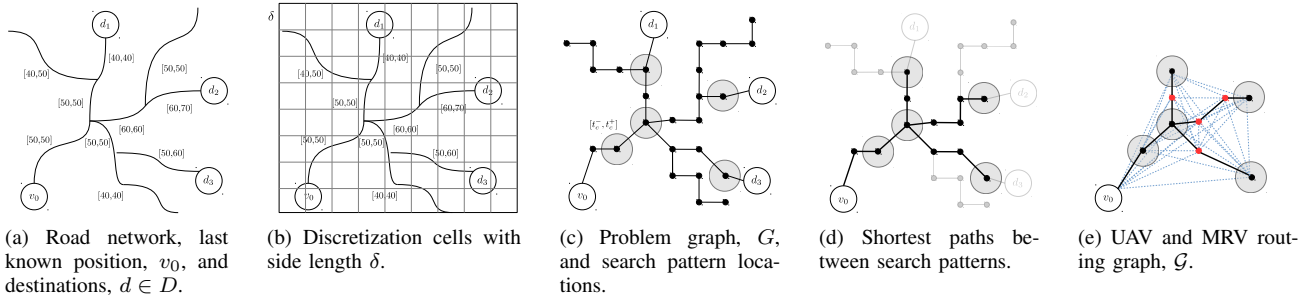
Fig. 1. UAV and MRV routing graph construction pipeline.
